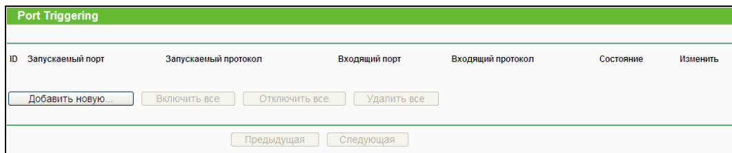
Рис. 4-48 Port Triggering
