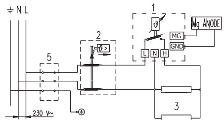
Electric installation
